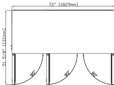
EDUR(F)72-B Top
