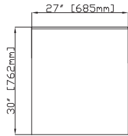
EDWR(F)27-B Front
