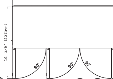
EDWR(F)72-B Top 72" [1829mm]
