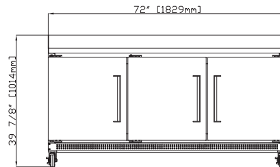
EDWR(F)72-B Front
