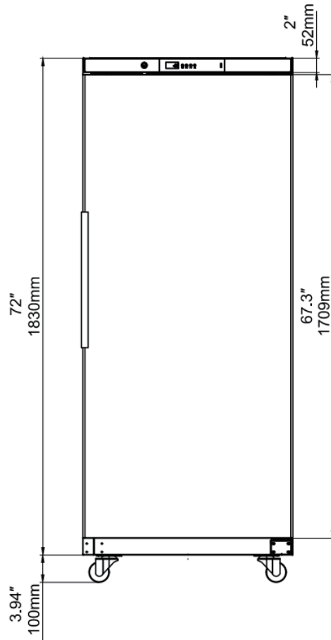
FRONT VIEW
