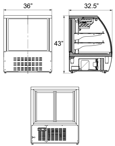
BSDC-36
