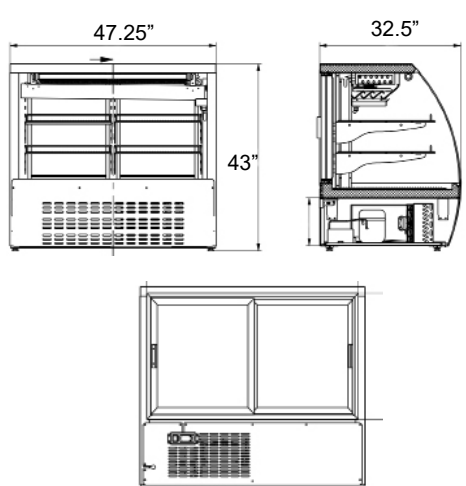
BSDC-48
