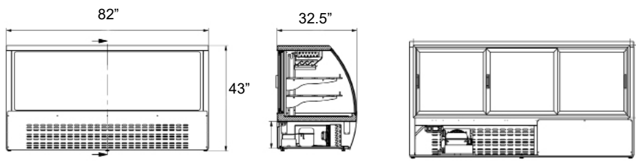
BSDC-82
