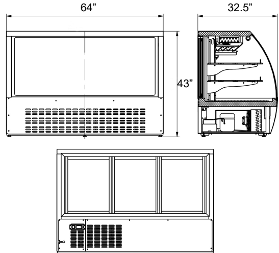
BSDC-64
